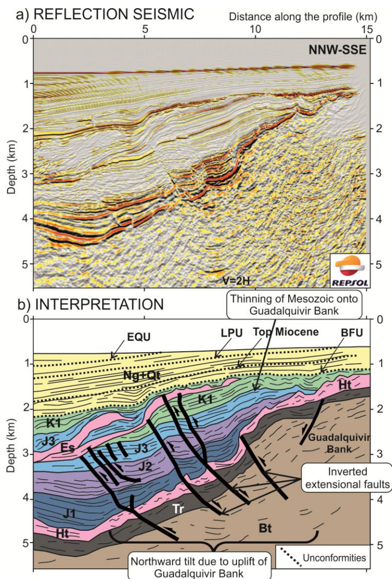
Figure 9. Reflection seismic profile in depth across the northern flank of the Guadalquivir Bank and the southwestern portion of the Esperança Salt (a), and its corresponding interpretation (b). See Figure 5 for legend. The section is the southern portion of a NNW-SSE trending section through the 3D seismic survey shown in Figure 3 (the precise location is not shown due to confidentiality). BFU = Basal Foredeep Unconformity; LPU = Late Pliocene Unconformity; EQU = Early Quaternary Unconformity. Data courtesy of Repsol.
