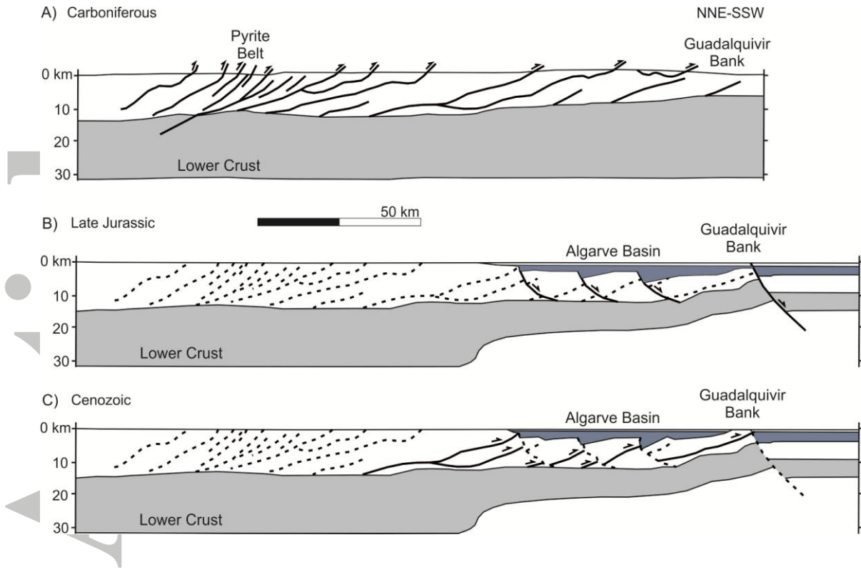
Figure 16. Synthetic crustal cross-section of the SW Iberian Margin at key time steps. (a) At the end of Variscan thrusting (Carboniferous). (b) At the end of Jurassic extension. (c) During Cenozoic thrusting. Black lines show faults active at each time step. Dashed black lines show inactive faults. Modified after Vegas et al. [2004].
