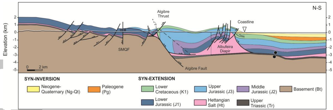
Figure 4. Cross section along the onshore Central Algarve Basin. Extensional motion on the southward-dipping Algebre Fault from Jurassic to Cretaceous times was responsible for the formation of the rollover structure, later inverted during Cenozoic compression. Inversion also led to the formation short-cuts and inversion of extensional faults in the northern sector of the figure. Notice the Algebre Thrust detaching on the Hettangian evaporite unit in the footwall of the Algebre Fault. Modified after Ramos et al. [2016]. See Figure 3 for location.
