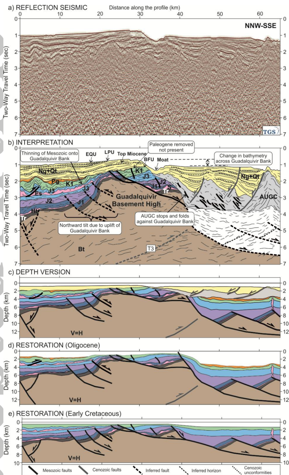
Figure 8. Seismic section across the Guadalquivir Bank. (a) Reflection seismic profile in time. (b) Interpretation of the same profile. (c) Depth version of profile in (a). (d) Restoration at Oligocene time (prior to the emplacement of the AUGC). (e) Restoration at Early Cretaceous time. The interpretation beneath the depth of 3-4 seconds is based on the 3D seismic image north of the Guadalquivir Bank and inferred to its south due to the
