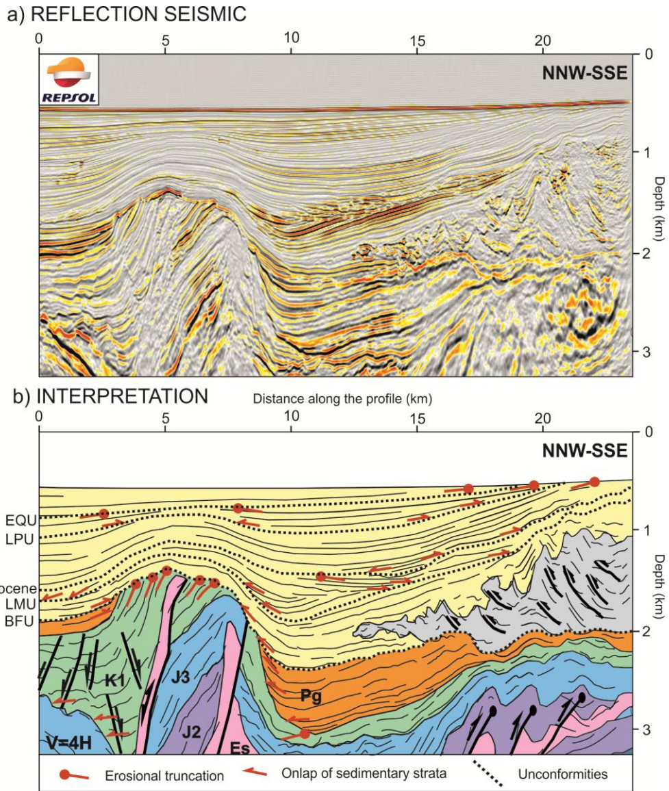
Figure 6. Seismic section of the detailed Cenozoic unit over the Esperança Salt in Figure 5 (a). Seismic interpretation showing the main unconformities within the Cenozoic sediments described by Hernández-Molina et al. [2016], along with the onlaps and erosional truncations resulting from different tectonic pulses (b). See Figure 5 for legend. BFU = Basal Foredeep Unconformity; LMU = Late Miocene Unconformity; LPU = Late Pliocene Unconformity; EQU = Early Quaternary Unconformity.
