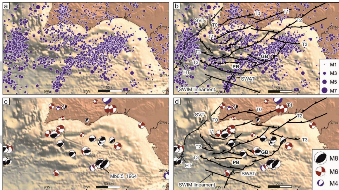
Figure 15. (a) Earthquake epicenters in SW Iberia, sized as a function of magnitude (modified after Palano et al. 2013). The earthquakes were recorded between 1951 and 2010, with magnitudes between 2.0 and 8.0 down to ~30km depth. (b) Location of the earthquake epicenters relative to the thrusts described in this paper. (c) Lower hemisphere, equal area projection for fault plane solutions, compiled from several earthquakes; red for strike-slip faulting, black for thrust faulting and blue for normal faulting, modified after Palano et al. [2013]. (d) Location of the focal mechanisms relative to the thrust faults described in the paper. GB: Guadalquivir Bank; PB: Portimão Bank; HT: Horseshoe Thrust; SVT: São Vicente Thrust; SWAT: South West Algarve Thrust.
