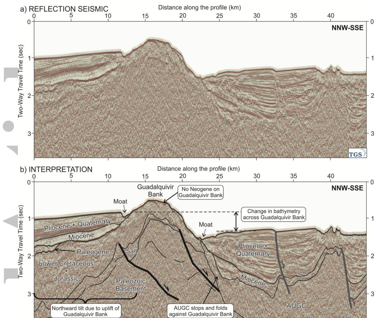
Figure 7. Seismic section across the Guadalquivir Bank in TWTT (a) and interpretation (b). Note the bathymetric relief of the Guadalquivir Bank and its lack of inner reflectivity. The onlap of Miocene to Quaternary sediments on both flanks indicates the presence of pre-Miocene sediments at seabed on the Guadalquivir Bank. Note also the northward tilt of sediments on the north of the Bank and the southward steepening of the AUGC and Miocene sediments on the south. See Figure 3 for location. Data courtesy of TGS.
