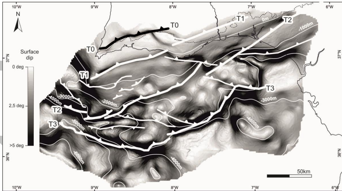
Figure 13. Map of the BFU colored for dip, with white contours indicating depth below sealevel. Steeper parts of the surface indicate steps in the surface, interpreted to be related to erosional geometries or to the presence of underlying basement-involving blind thrusts (traces of the thrust tips shown in white lines).
